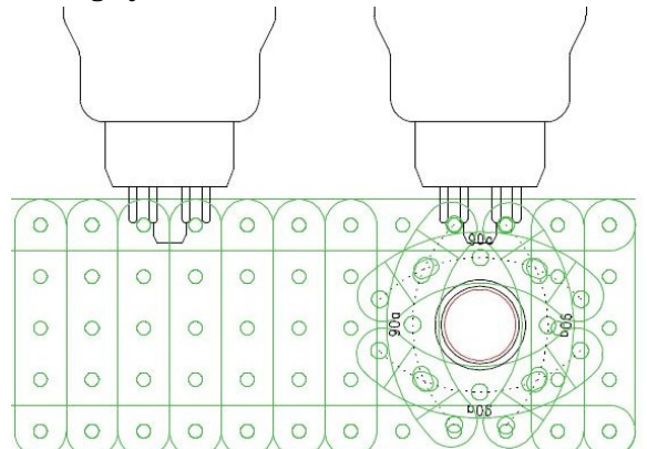
Working out details to mount the ¾” diameter front panel indicator recuperated from the old Trix amp using 90As.
