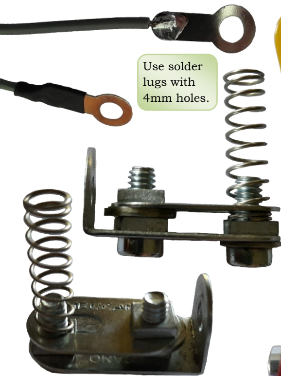
From Tim Gant. Mounting an N20 motor using only standard parts. No filing or drilling. Yet again we find that Frank Hornby had all the answers without going off into the wilderness.
