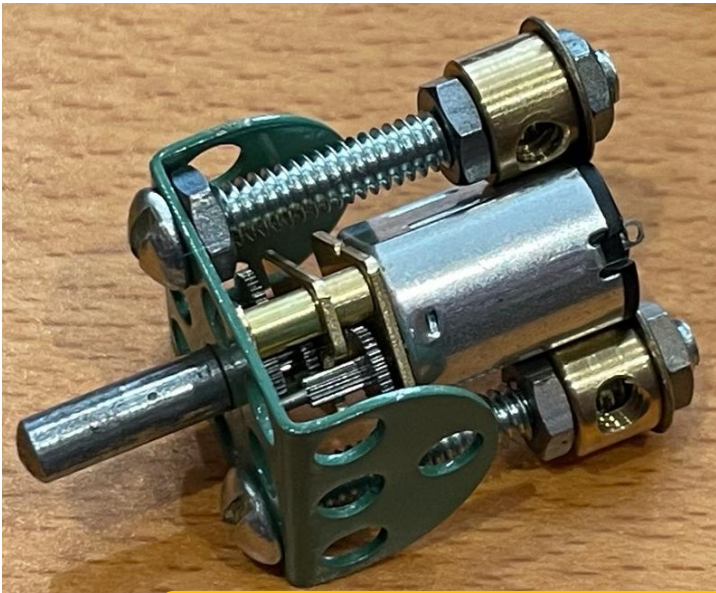
From Tim Gant. Mounting an N20 motor using only standard parts. No filing or drilling. Yet again we find that Frank Hornby had all the answers without going off into the wilderness.
