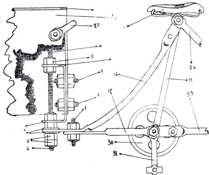
Motor unit resembling Pivot for delivery tricycle Sprocket wheel of bottom bracket Falso motore Sostegno del tri porteur Pedaliere
