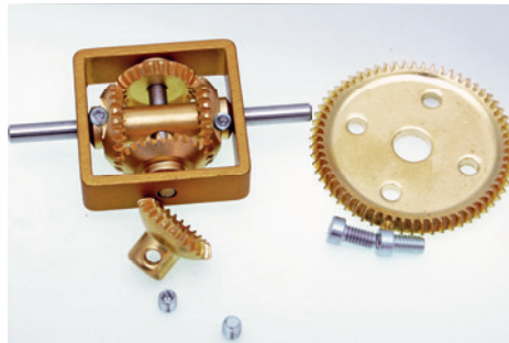
BG05 | Differential Set
