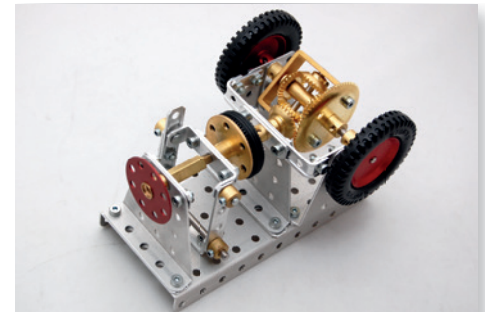
BG04 | Differential m. Kupplung
